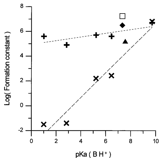
Figure 7. Plot of \log \beta_2^{\text{II}} and \log \beta_2^{\text{III}} for the iron tetrphenylporphyrinate complexes of this study versus the basicity of the axial ligands, expressed as pK_a(\text{BH}^+) : +, substituted pyridines, \text{Fe}(\text{II}) ; x, substituted pyridines, \text{Fe}(\text{III}) ; □, N -MeIm, \text{Fe}(\text{II}) ; ◆, N -MeIm, \text{Fe}(\text{III}) ; ▲, 2-MeImH, \text{Fe}(\text{III}) . Dashed lines represent the least-squares linear correlations for the substituted pyridine complexes of \text{Fe}(\text{II}) and \text{Fe}(\text{III}) .
